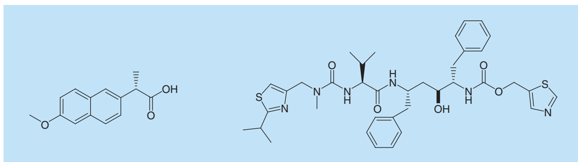
Figure 1. Molecular structures of naproxen (left) and ritonavir (right).
